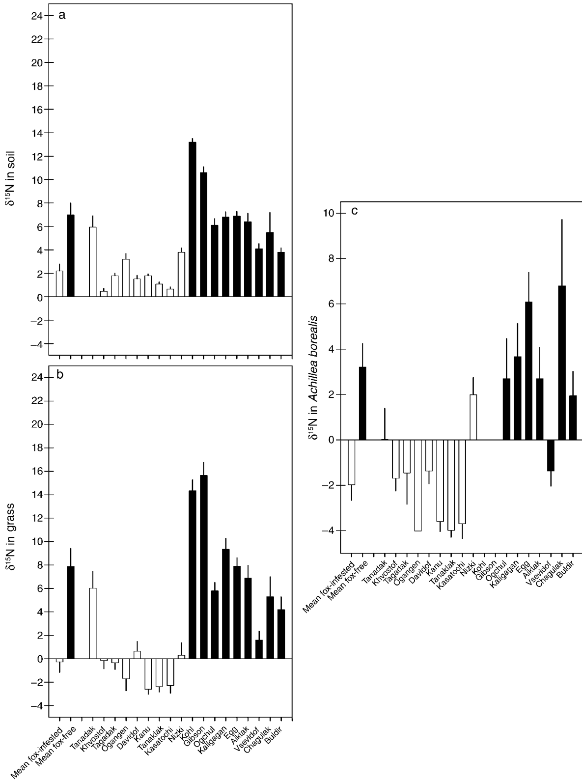
FIG. 3. Content of \delta^{15}\text{N} (mean \pm SE) in (a) soil and (b) grass, and (c) Achillea borealis on fox-free (black bars) and fox-infested (open bars) islands. Within island type (i.e., fox-free or fox-infested), islands are arranged from left to right, in order of smallest to largest size.
